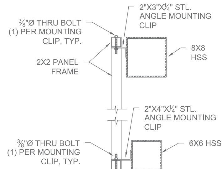
TYP. PANEL FRAME TO ARCH CONNECTION
